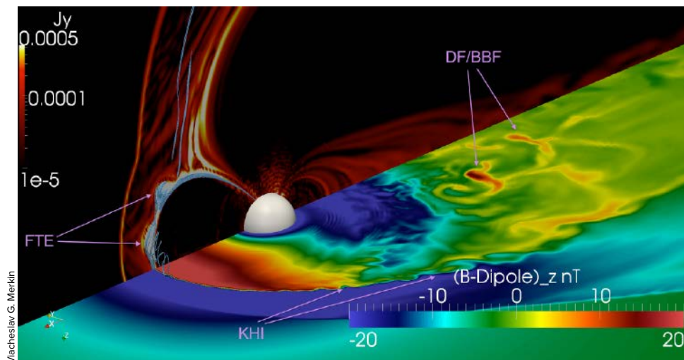
Dipolarization fronts (DFs), bursty bulk flows (BBFs), flux transfer events (FTEs), and Kelvin-Helmholtz instability (KHI) in a high-resolution simulation of an idealized substorm. The simulation was performed using the Lyon-Fedder-Mobarry global magnetosphere model.
