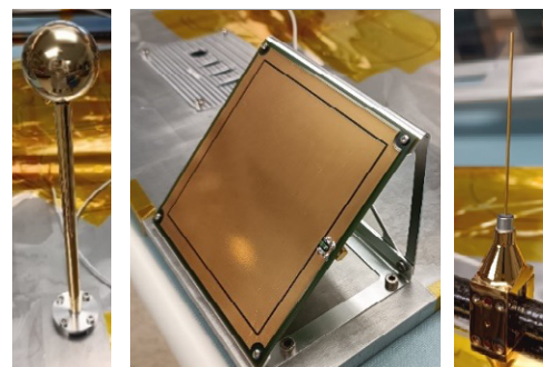
The ESCAPE Langmuir Probe suite includes a Floating Potential Probe (left), Planar Ion Probe (middle), and multi-Needle Langmuir Probe (right). Credit: A. Barjatya (Embry-Riddle Aeronautical University)
