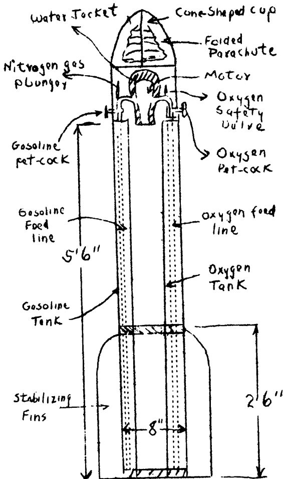
Schematic drawing of the Rocket of A.I.S. Length overall 7 feet
