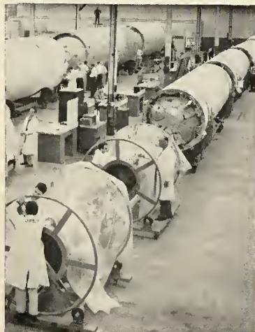
JUPITER AND REDSTONE ballistic missiles move down parallel production lines at the Warren Missile Plant of Chrysler. The number of Jupiters shown indicates quantity production is being achieved. A Jupiter tank assembly undergoes dynamic tests at the missile plant (right). The missile section has been lowered into a test pit below the floor level for this operation. Heavy presses and other production equipment used for manufacture of components can be seen in the background.
