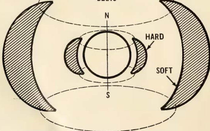
Figure 3 EARTH'S RADIATION BELTS
