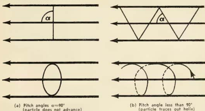
Figure 1 PARTICLE MOTION AND REFLECTION IN MAGNETIC FIELD
