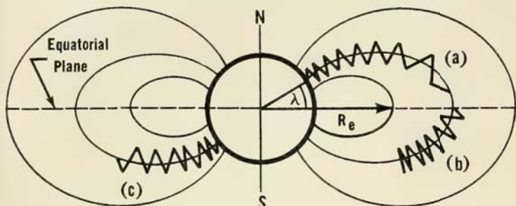
Figure 2 PARTICLE TRAPPING IN EARTH'S MAGNETIC FIELD
