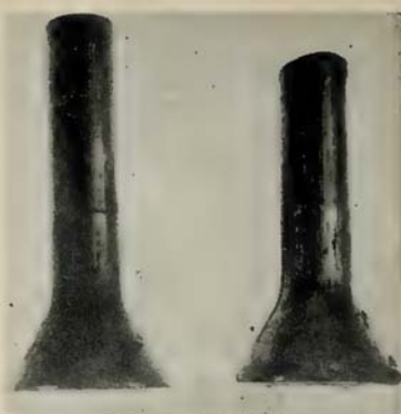
IMPACT extrusions of columbium-base alloys permit normal fabrication.
