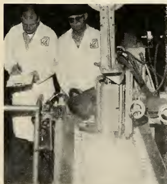
SIGMA welding is used by Reynolds Metals to make longitudinal weld on Redstone 's center section.
