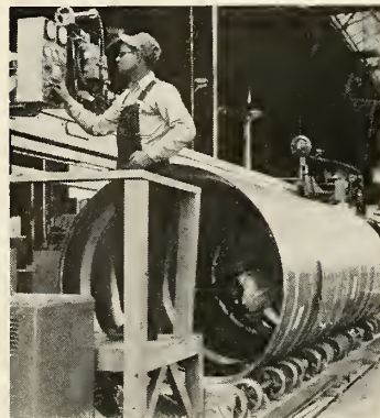
ANOTHER Sigma machine makes a girth weld on Redstone fuel tank.
