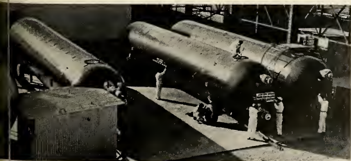
STANDARD STEEL Corp. is delivering vacuum-jacked LOX tanks for Thor . Holding 13,500 gallons, the 52' tanks have a high-strength aluminum outer jacket and a stainless steel inner shell.
