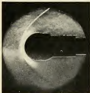
HOT GAS gap generated at high speeds created with 2500 kw AC air-stabilized free jet, proved out models.
