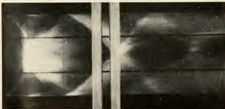
STREAK PHOTOGRAPH of cylindrical pinch was taken through 0.05 slit in upper electrode.
