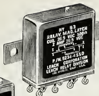
(STUD MOUNTING, SOLDER HOOK TERMINALS, HERMETICALLY SEALED)
