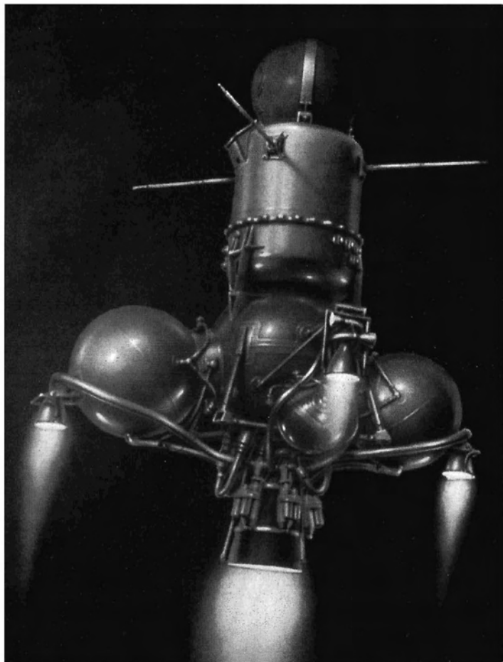
► Clockwise from left: The Luna 16 spacecraft was the first vehicle to land on the Moon, collect a soil sample, and return to Earth; an artist's impression of Luna 16 lifting off the lunar surface with its precious cargo; Lunokhod 1 was driven around the lunar landscape for 11 months by Earth-based controllers.
