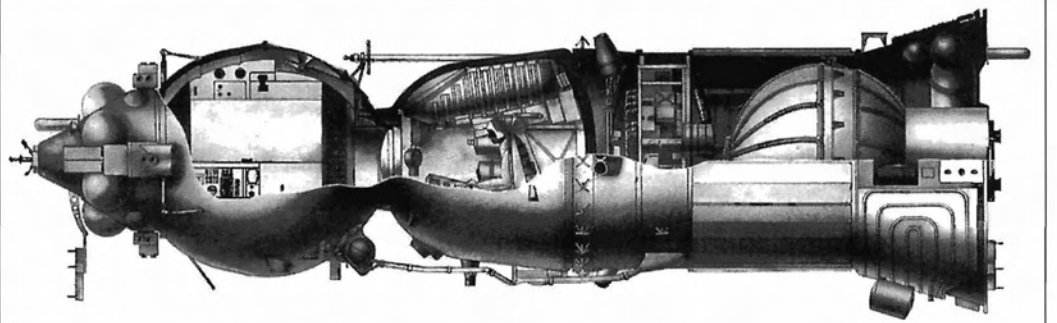
► Top: The Soyuz 4/5 crew transfer in Earth orbit during January, 1969, was necessary to demonstrate the technique which the LK cosmonaut would employ twice in lunar orbit. Right: The LOK lunar orbiter. Bottom: The LK lunar lander weighed 5.5 metric tons.
