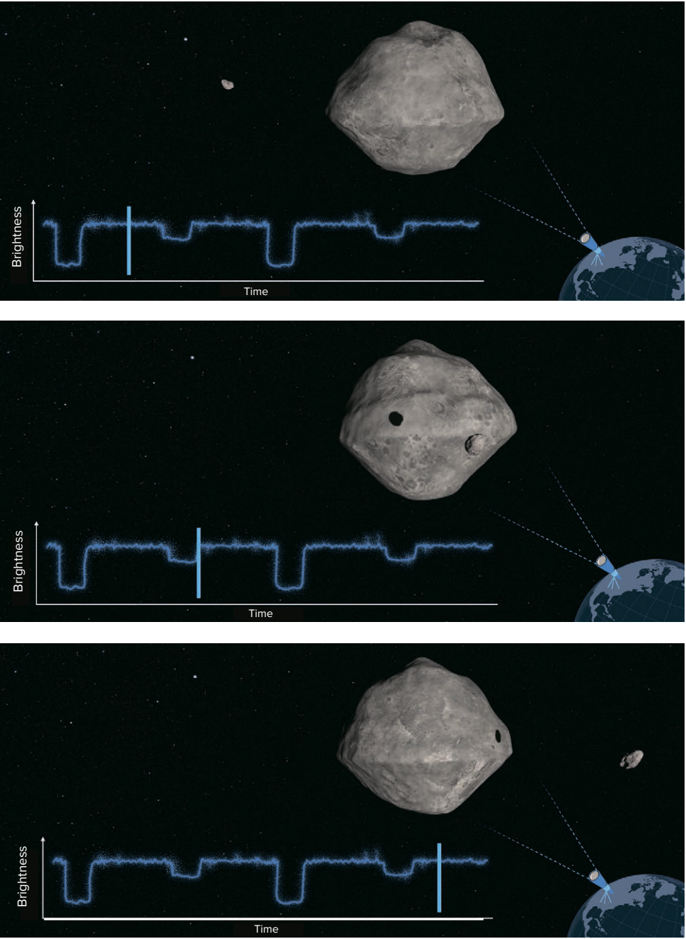
Dimorphos Orbiting About Didymos
