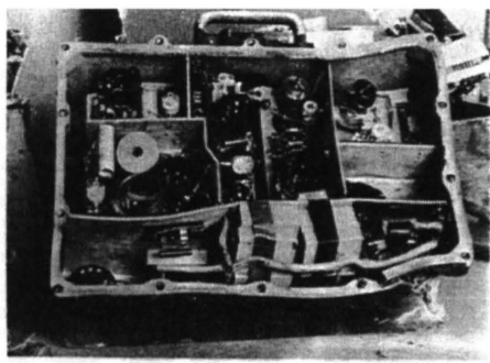
Figure 10-5c: Reconstruction at FFA. Receiver and transmitter. Credit: Kjellson, Ref. 9.
