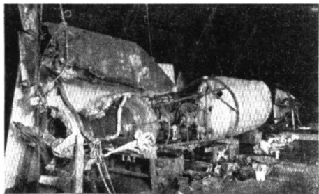
Figure 10–13: Reconstruction of the A4/V-2 No. V89 from Sweden at Farnborough. Credit: Ref. 15.
