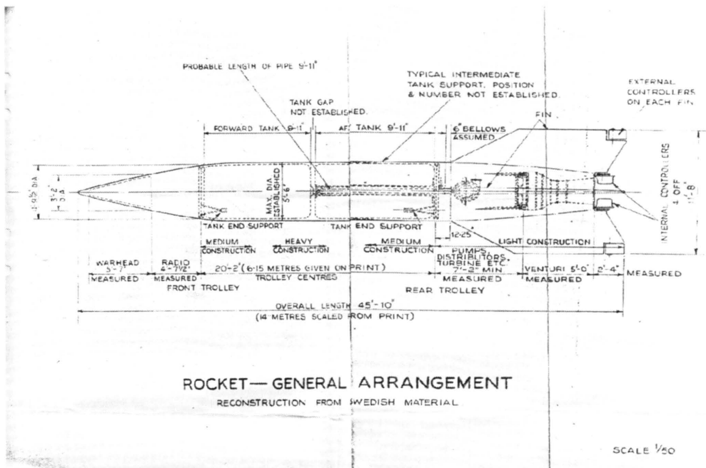
Figure 10-14: Drawing in RAE report EA 228/6, dated 18 August 1944. Credit: Ref. 13.
