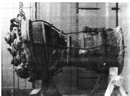
Figure 10-5b: Rocket engine reconstruction at FFA. Credit: Kjellson, Ref. 9.
