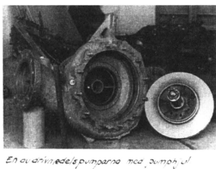
Figure 10–8: One of the propellant pumps, Ø 270 millimeters. Credit: Kjellson, Ref. 9.
