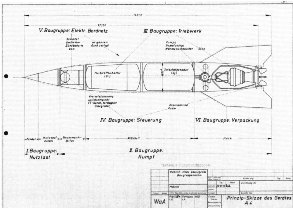
Figure 10-15: Official German Drawing of the A4 from 1941. Credit: BArch RH 8-1350, Germany.
