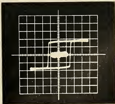
SQUARE HYSTERESIS loop of magnetic rod. Ratio is better than 0.95.
