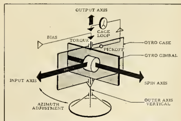
SINGLE AXIS gyro showing input, output and spin axes.
