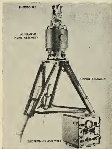
BASIC ELEMENTS of ABLE: alinement head; electronics; and tripod.
