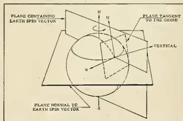
WHEN INPUT axis of gyro is horizontal, axis must be parallel to true E-W line.
