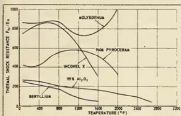
FIG. 4—Comparison of thermal shock resistance factor with steady-state temperature differentials.
