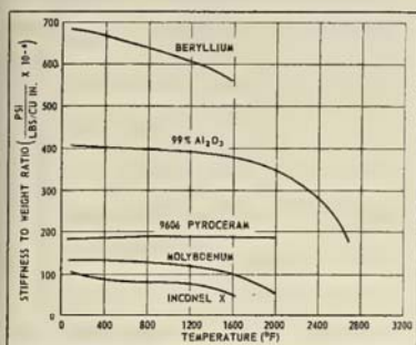
FIG. 3—The stiffness to weight ratio of metals vs. ceramics.
