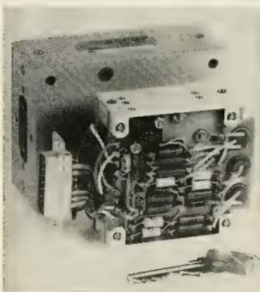
INTERIOR OF a K-Series transistorized Pulse Width keyer module, shown with outside casing, for coding the output.
