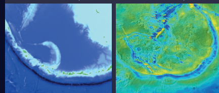
Aleutian trench, Earth Artemis corona, Venus
