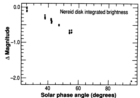
Fig. 41. Disk-integrated phase curve for Nereid. The photometric data were extracted from 15-exposures taken through the narrow angle clear filter during the last 12 days of approach.
