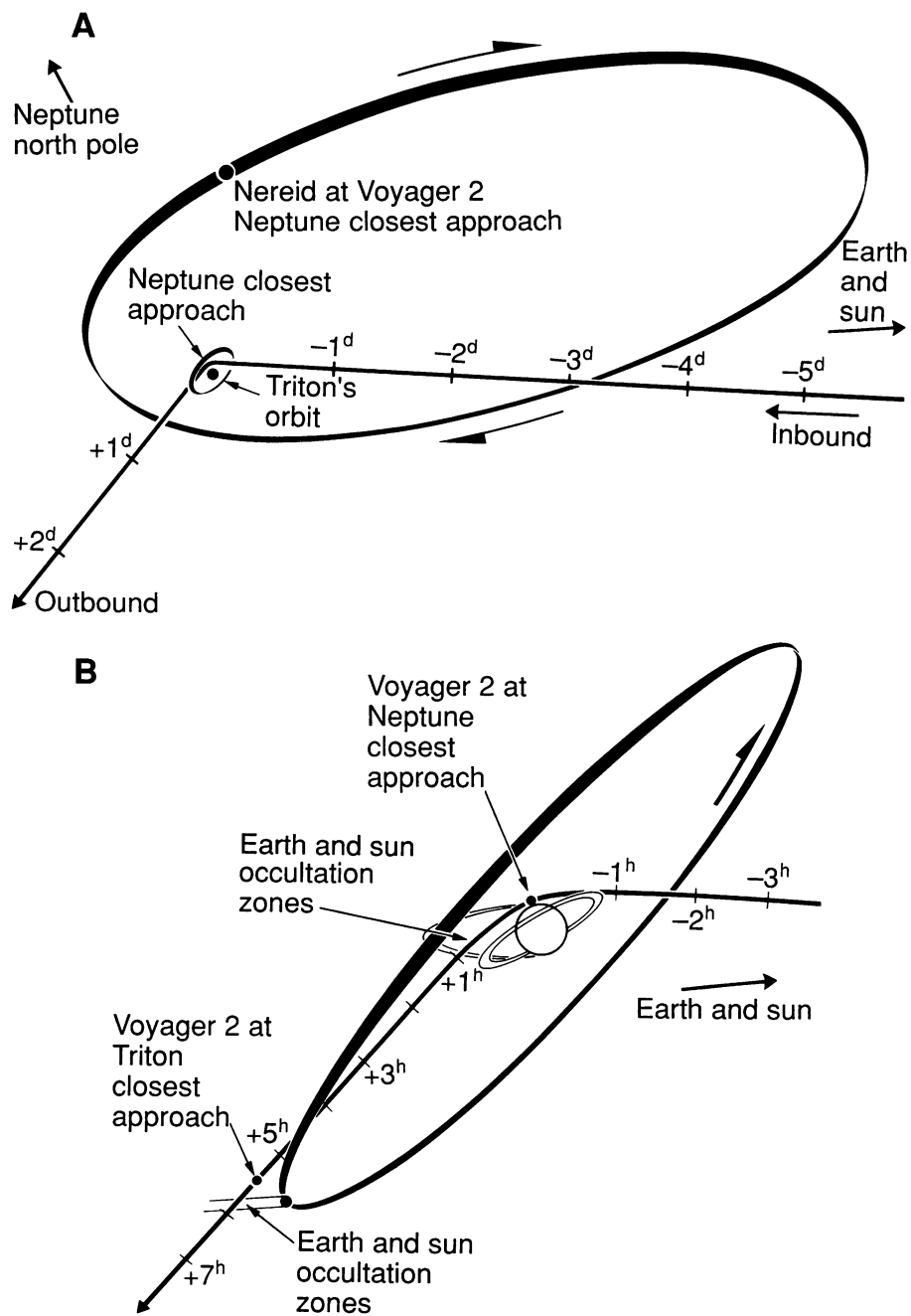
Fig. 1. The Voyager 2 path through the Neptune system is shown in the plane of the spacecraft trajectory. (A) The projected orbits of Triton and Nereid are shown, together with the positions of these satellites at the time of Voyager 2's closest approach to Neptune. Tick marks along the trajectory indicate Voyager's position at 1-day intervals. (B) An enlarged view covers a 10-hour period that includes closest approaches to Neptune and Triton and passage through Earth and solar shadows (occultation zones) of each. Tick marks along the trajectory are at 1-hour intervals.
