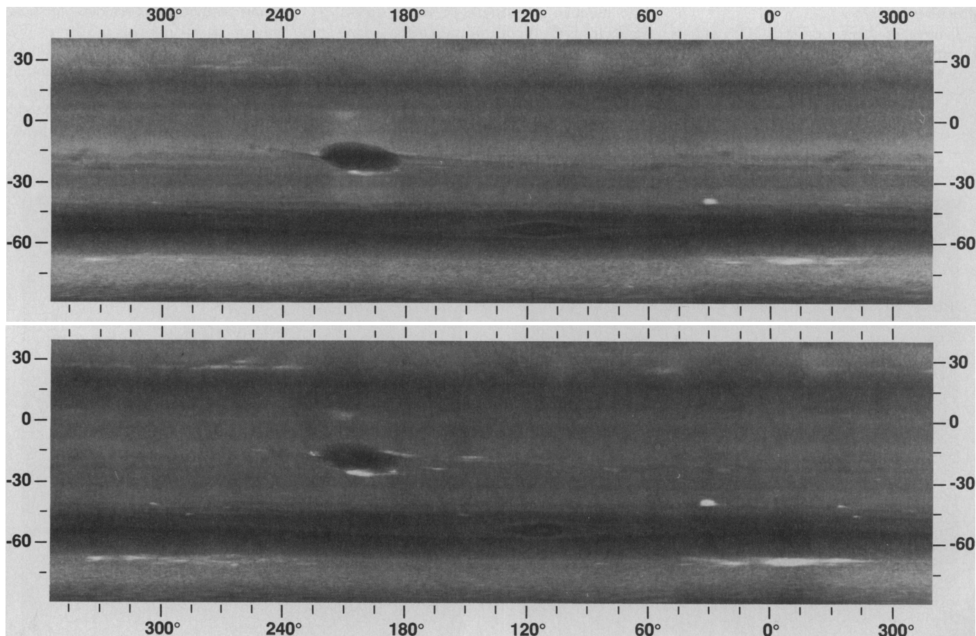
Fig. 2. Simple cylindrical projection mosaics of narrow-angle images taken through the blue ( top ) and green ( bottom ) filters on 17–18 August 1989. Latitude is planetocentric and longitude is based on a rotation period of 17 hours 52 min, the “predict” period used to plan Voyager observation sequences. This is longer than the 16.1 hour period derived from the Planetary Radio Astronomy investigation (3). For each mosaic, approximately ten images were shuttered, during which time the planet rotated through slightly more than one rotation. Thus features visible near the right
