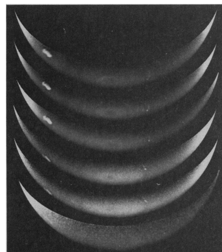
Fig. 7. Neptune's bright crescent taken in six filters (from bottom to top: UV, violet, blue, clear, green, orange) on 31.3 August 1989 (7). The images were shuttered in temporal order: violet, blue, UV, clear, green, orange. These images show the bright core of D2, the south polar feature, and the symmetric structure immediately surrounding the south pole. The relatively high contrast of the features in these images indicates that they extend above most of the scattering haze and absorbing methane gas in Neptune's atmosphere. [Image processing by D. A. Alexander]
