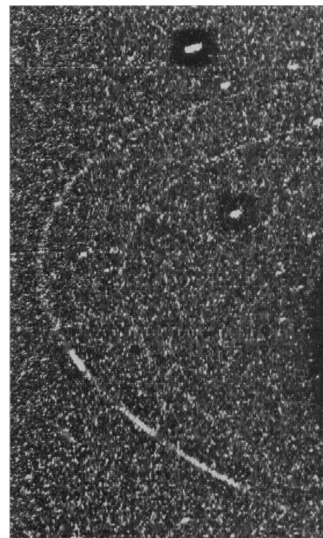
Fig. 16. This Voyager 2 image (FDS 11350.23), a 111-s exposure obtained through the clear filter of the wide angle camera, shows the N53 and N63 rings faintly in backscattered light (phase angle of 15.5°). Relatively prominent in the N63 ring are the three Neptune ring arcs. The satellite 1989N2 can be seen in the upper right corner, streaked by its orbital motion; the other bright object is a star. The arcs are unresolved in this image (resolution of 37 km per line pair); their apparent width is due to image smear.
