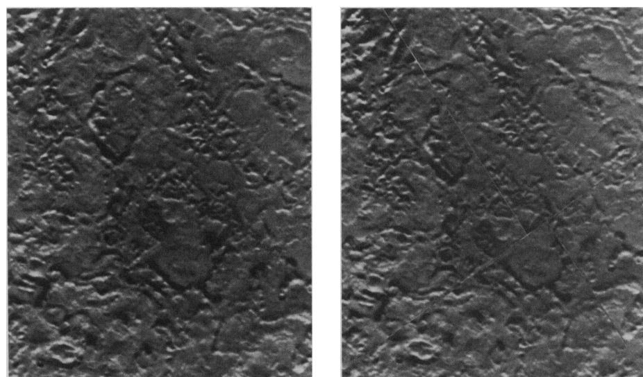
Fig. 32. Possible strike-slip faulting on Triton. ( Left ) The irregular depression near the center of the view appears to have been distorted by lateral faulting. ( Right ) One possible reconstruction of the feature shown in this view requires two episodes of strike-slip faulting, each with roughly 30 km of displacement.
